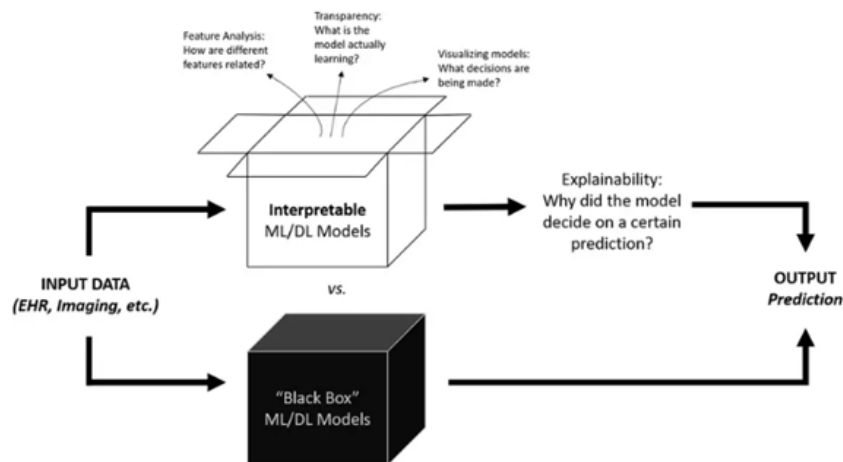
Figure 2.18: Black Box Concept vs. Explainable AI [41]
