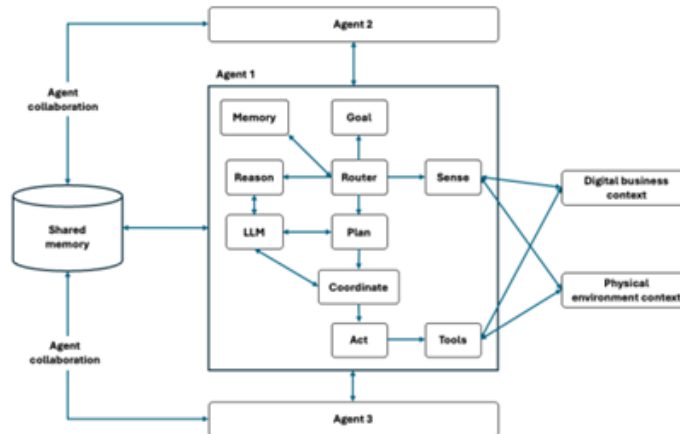
Figure 2.9: Agentic AI anatomy [24]
